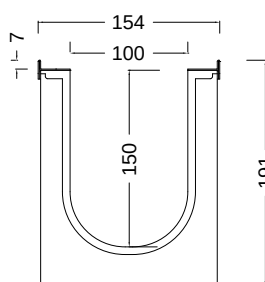
NEOMAX 100H 100/150
