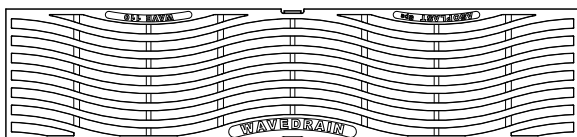
1 HDPE WAVE STYLE GRATING
