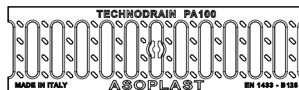
5 POLYAMIDE GRATING B125 18 mm
