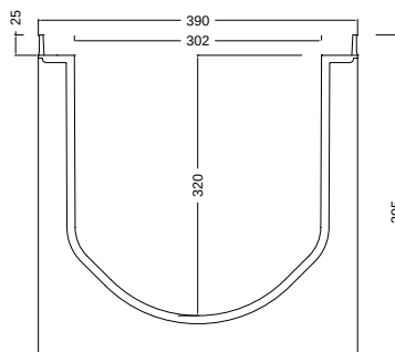
MAGNUM CITY 300/320
