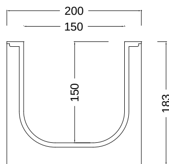
NEO 150H 150/150
