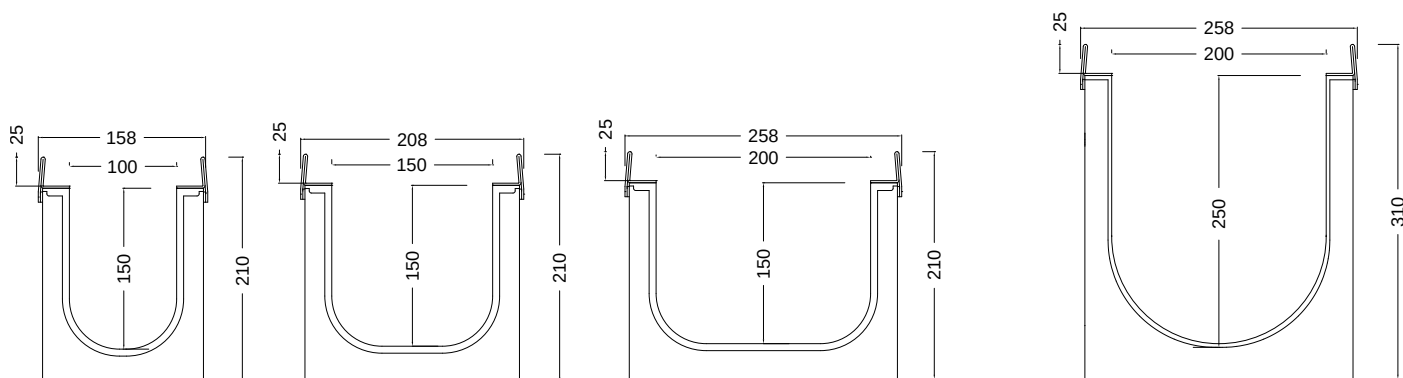
EXEL 100H 100/150
