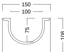
NEO 100S 100/75
