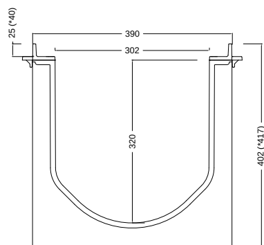
MAGNUM TRAFFIC 300/320
