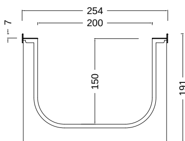
NEOMAX 200H 200/150
