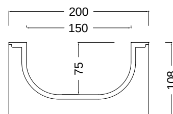
NEO 150S 150/75
