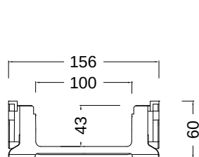
NEO 100SX 100/43
