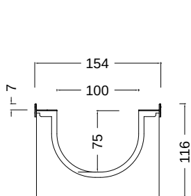
NEOMAX 100S 100/75
