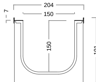
NEOMAX 150H 150/150
