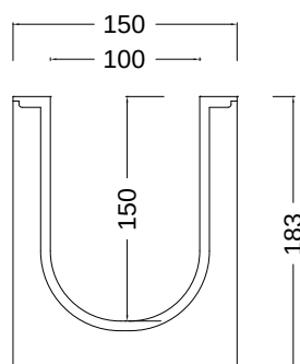
NEO 100H 100/150
