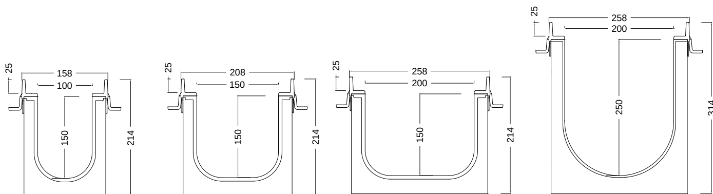
PROMAX 100H 100/150
