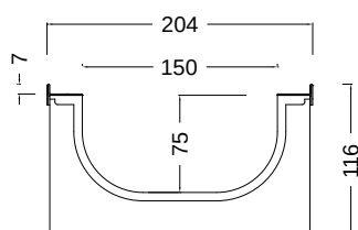
NEOMAX 150S 150/75
