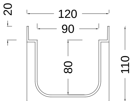
CHANNEL WAVEDRAIN 110
